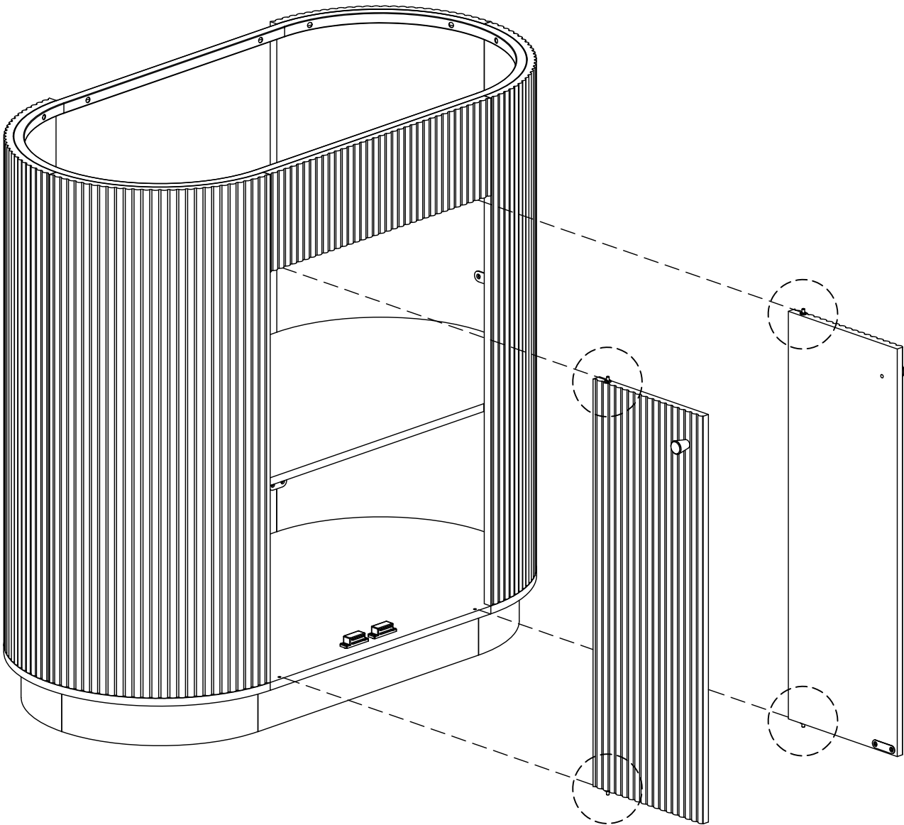
STEP2:Press and hold upper pivot pin #L, push the door under board #1, then slide the pin into the hole.
