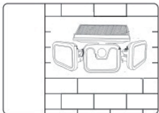
4. Hang the unit on the installed support frame corresponding to the holes behind the unit.
