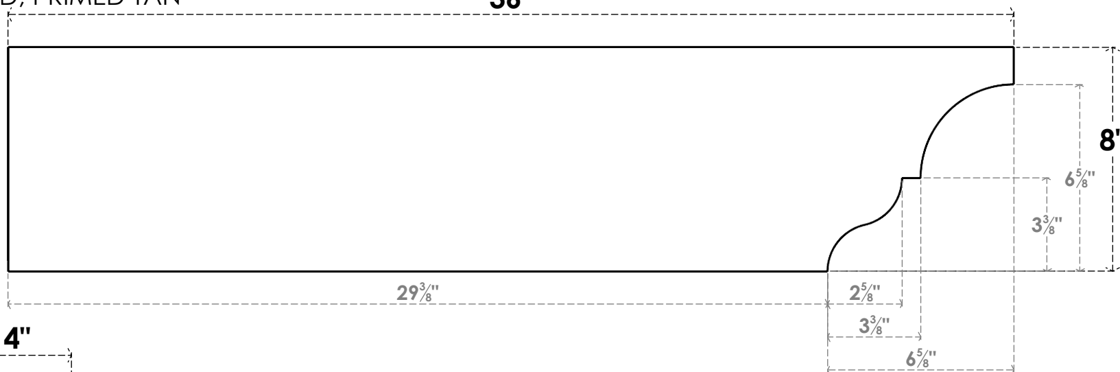
SIDE PROFILE
