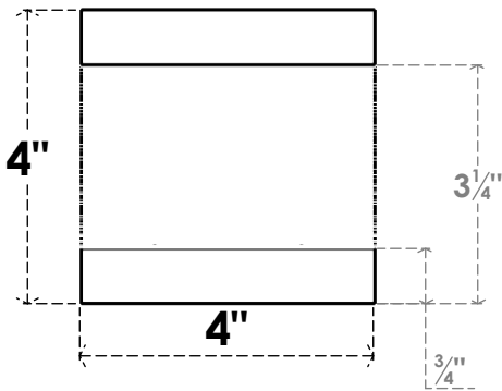
FRONT PROFILE
