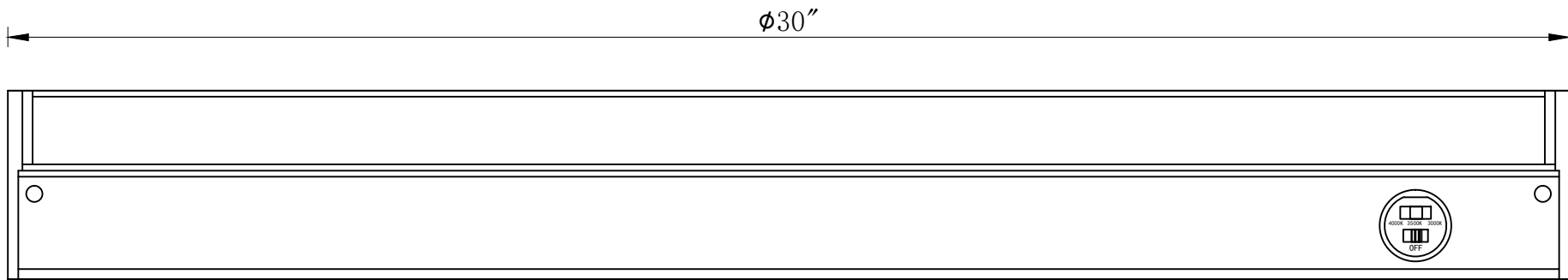
FRONT VIEW
