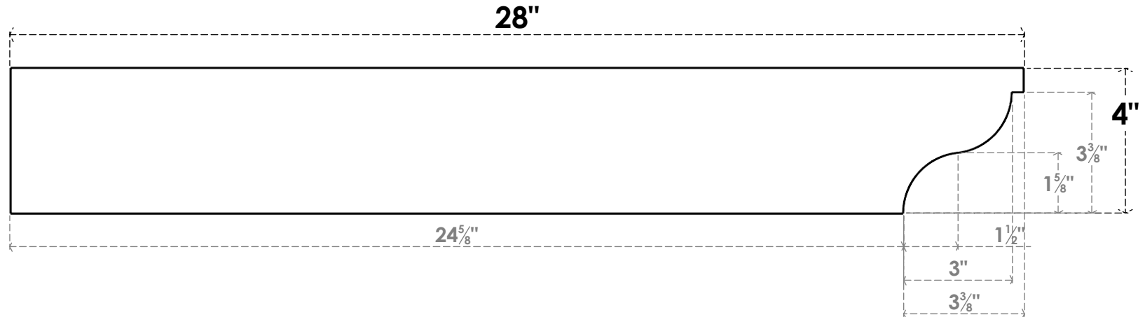
SIDE PROFILE
