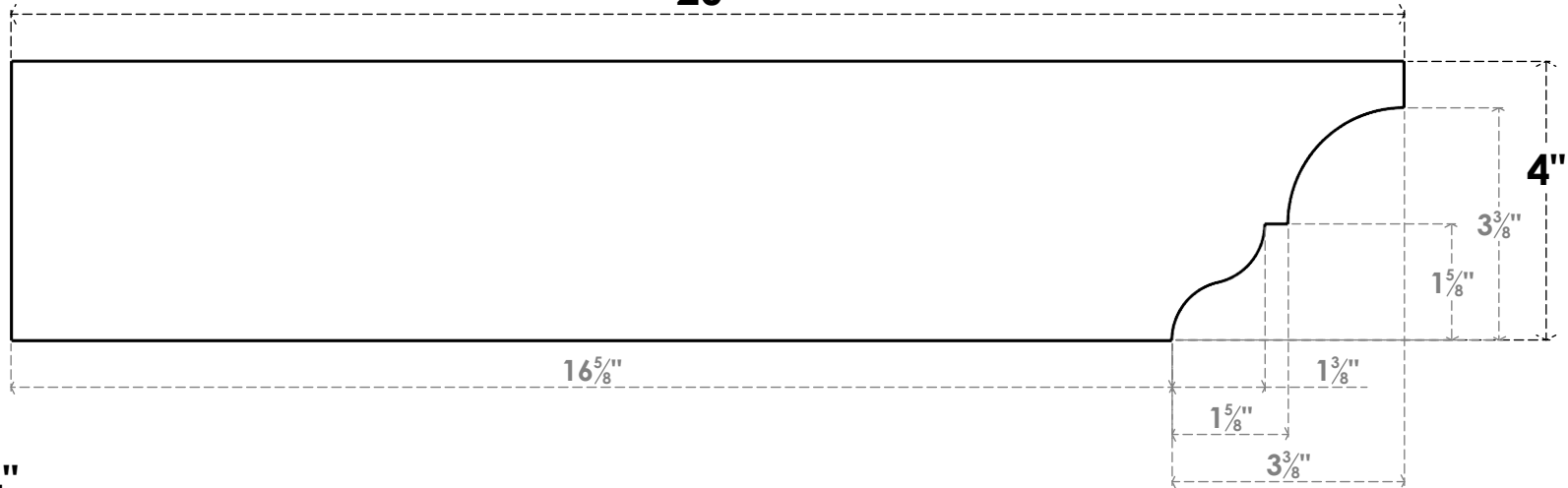
SIDE PROFILE
