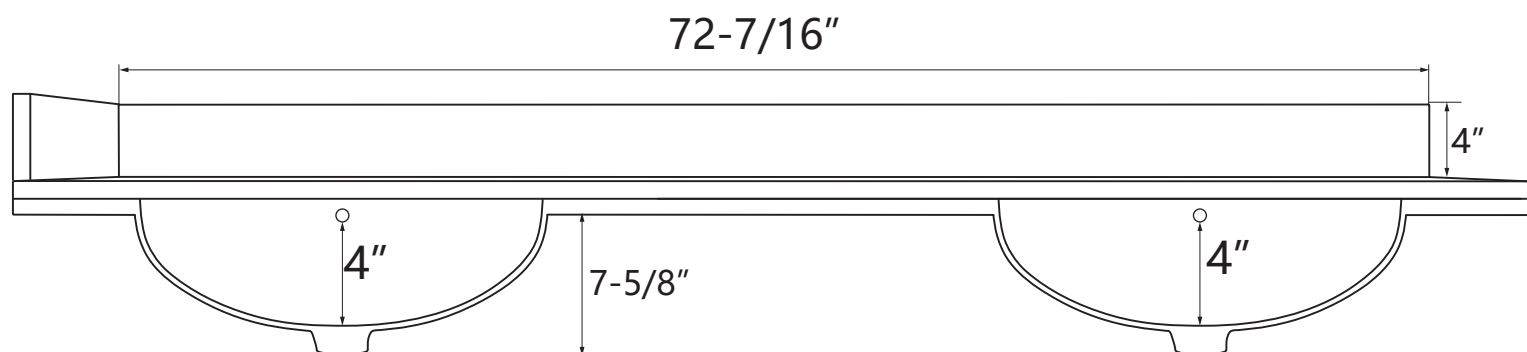
Front View
