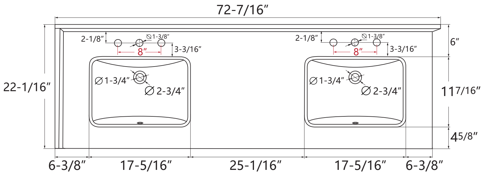
Top View
