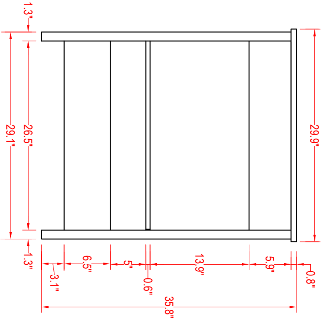
(BACK)
