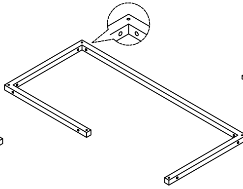
Bottom Frame
