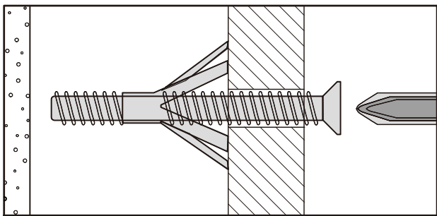
No.3 "Cavity Fixing" wall plug
