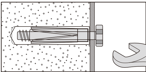
No.6 "Shield Anchor" wall plug - heavy loads
