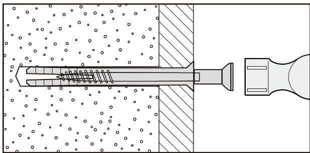
No.5 "Hammer Fixing" wall plug
