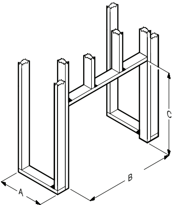
Framing Dimensions
