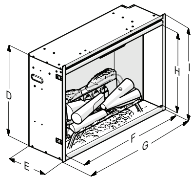
Firebox Dimensions
