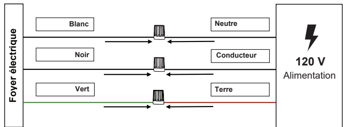
Figure 10 Câblage direct (120 V)
