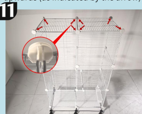
Step 11: Top sealing: Connect the top through the connecting buckle network
