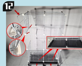
Step 12: Install one iron mesh door and insert it into the gap through the left and right buckle links. Push two pallets together and inside
