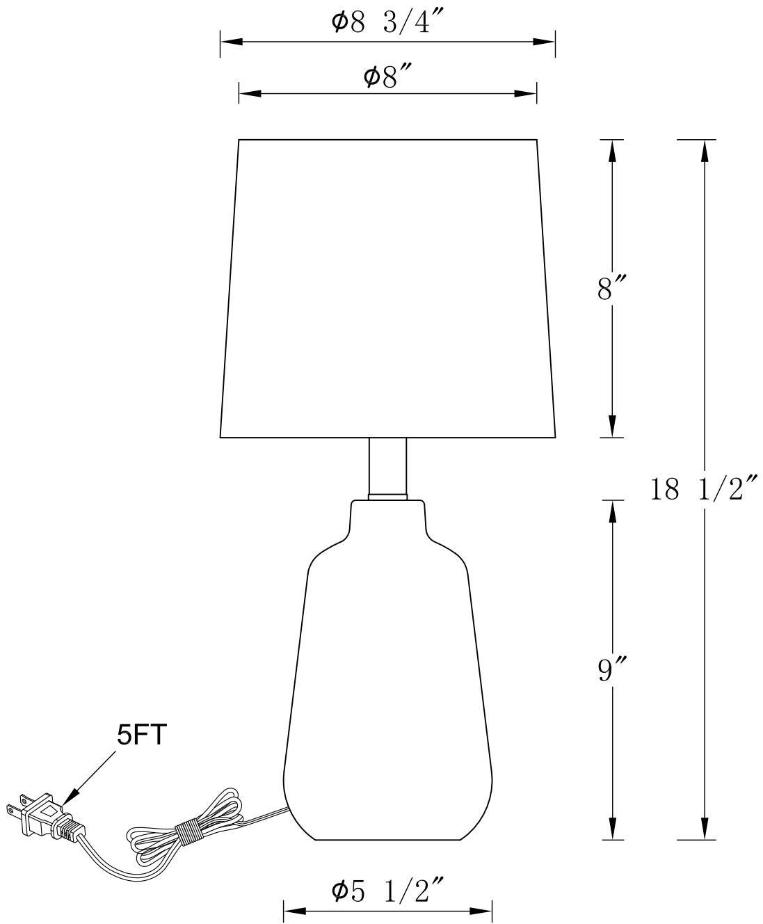
FRONT VIEW
