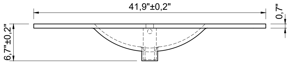
FRONT VIEW
