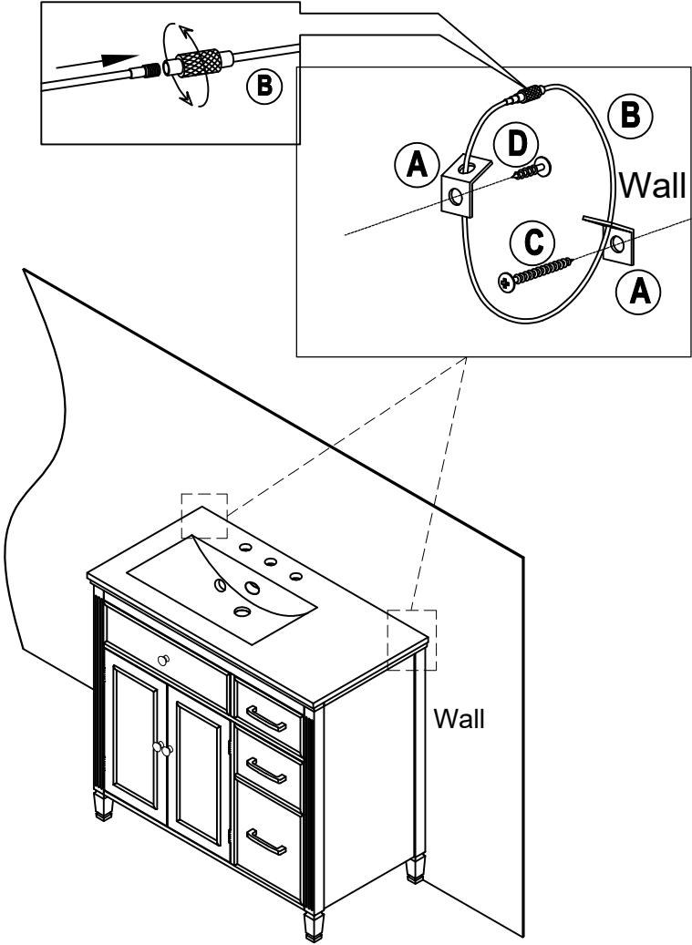
Hardware list: Anti fall hardware (2 sets)
