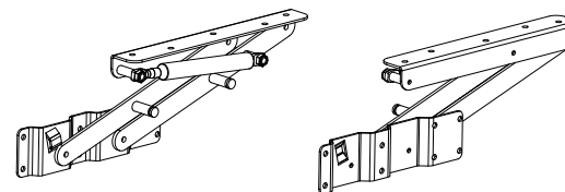
Lifting Mechanism
