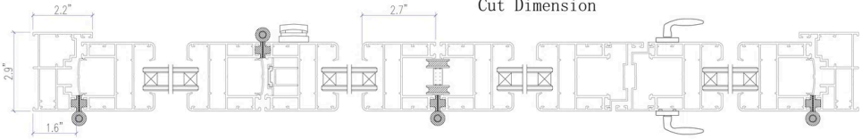
Cut Dimension
