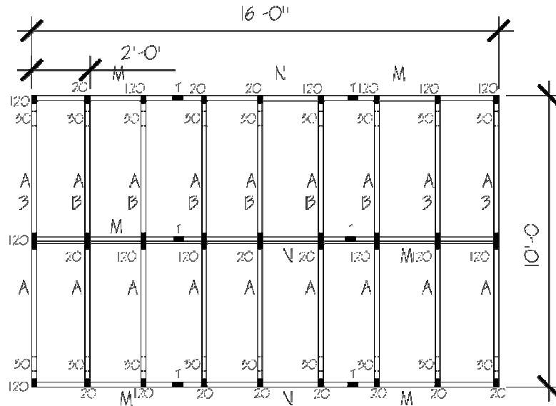
ROOF PLAN
