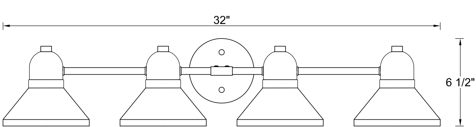
FRONT VIEW
