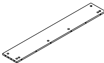
⑤ (968x156x12mm)X1
