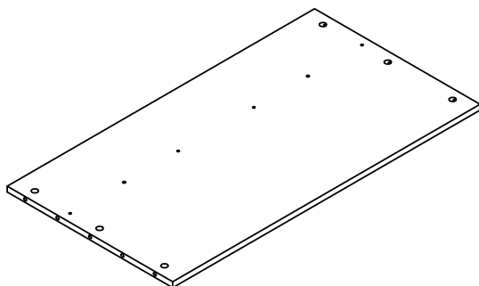
① (910x490x15mm)X1
