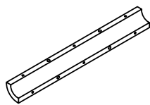
④ (490x63.6x26.2mm)X2
