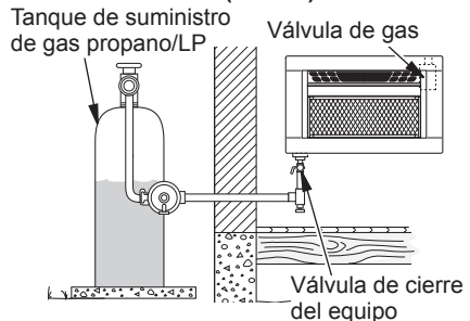
Figure 19 - Propano/LP suministro de gas
