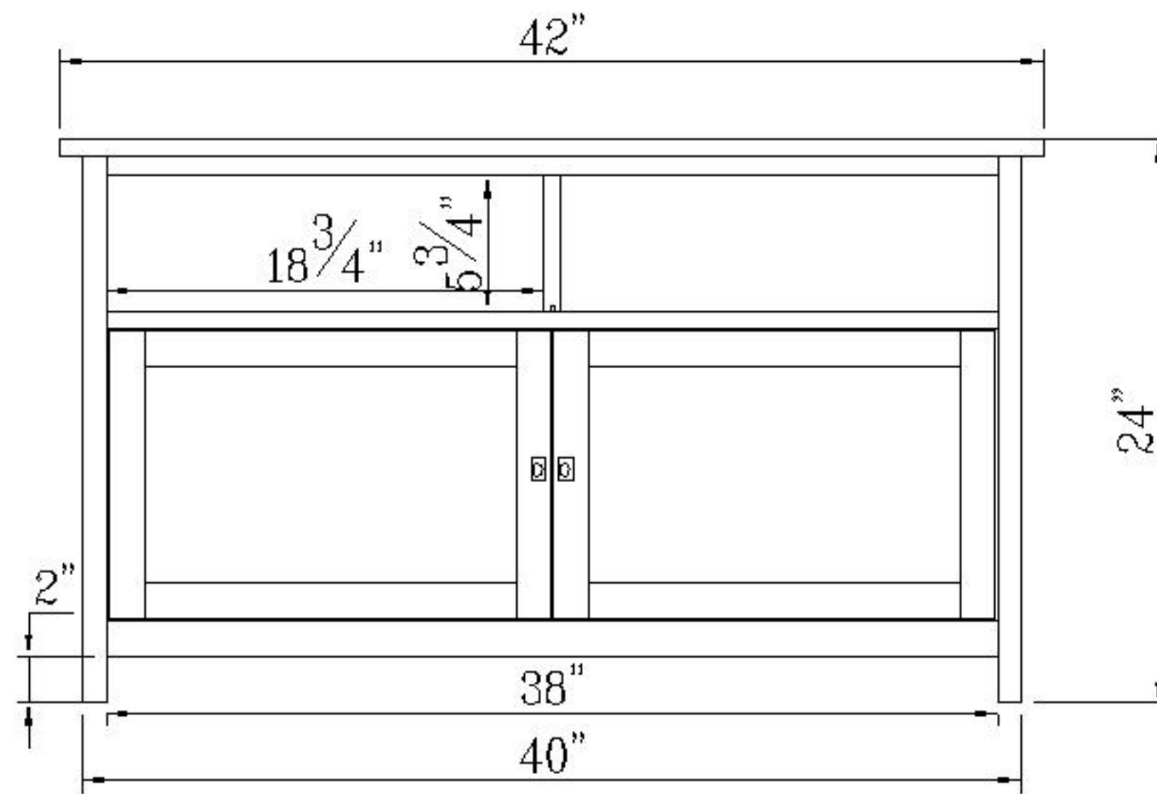
FRONT VIEW
