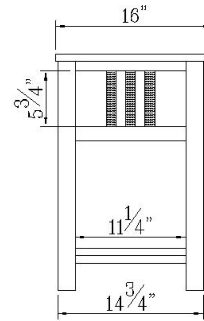
SIDE VIEW
