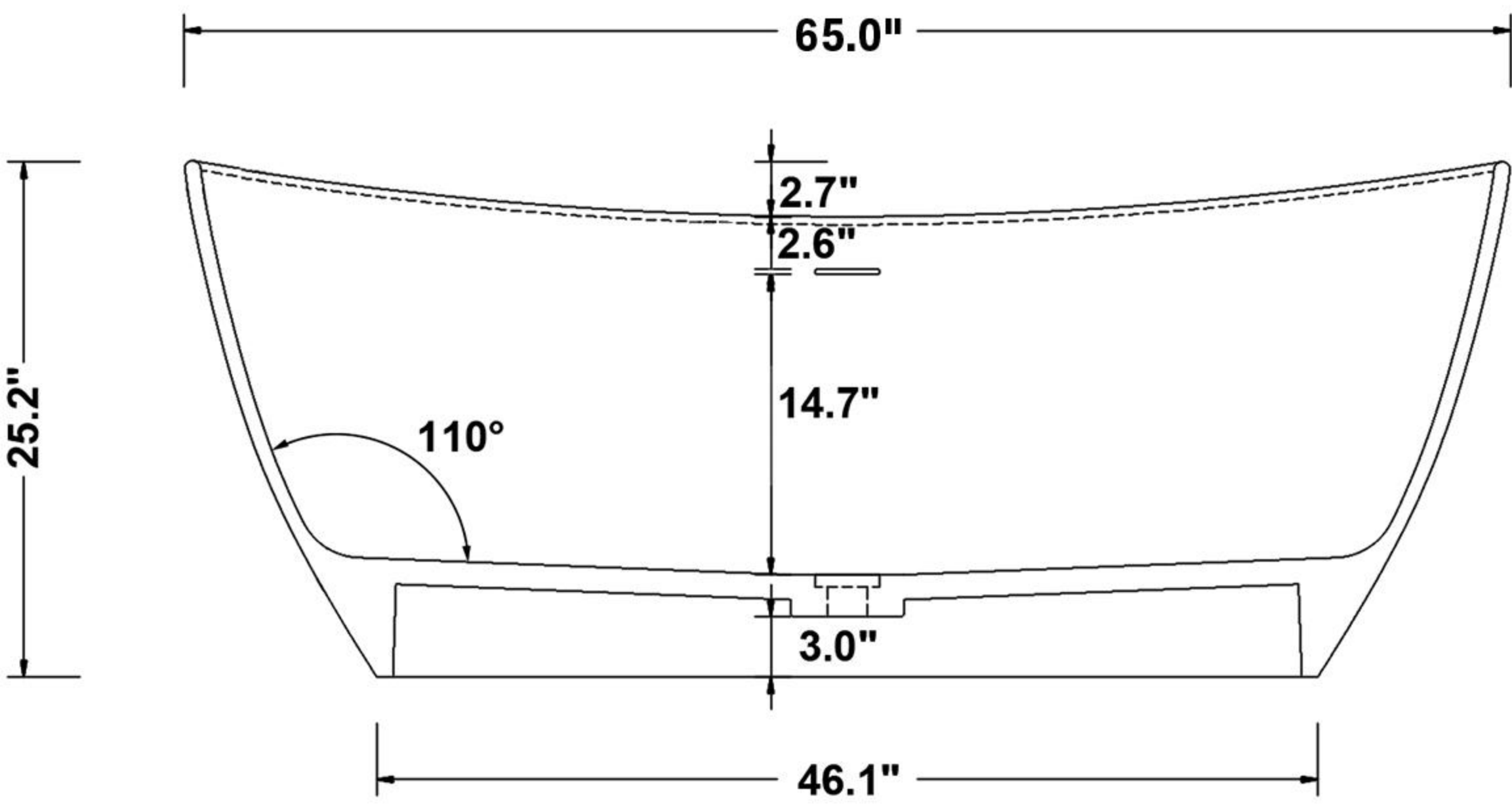
vertical view
