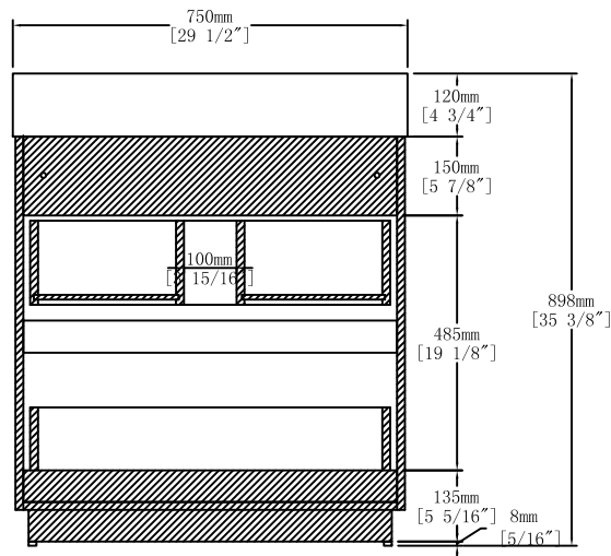
Back View
