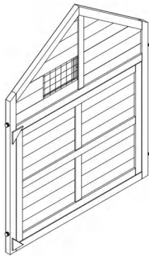
Front panel of coop 1PC
