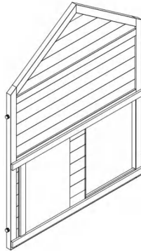
Back panel of coop 1PC
