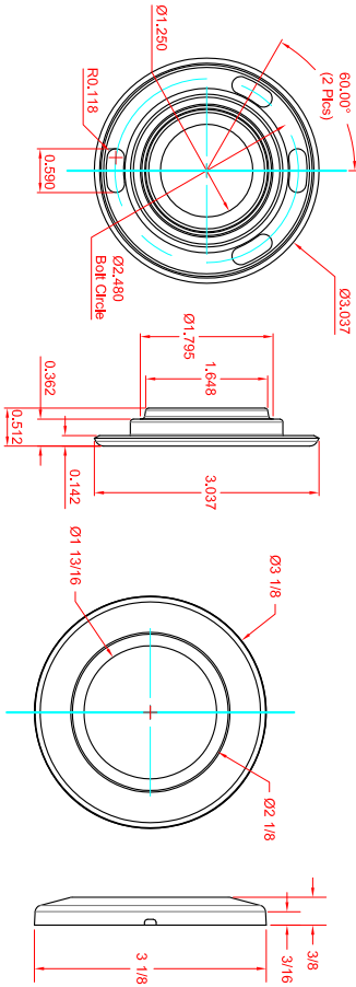
IFSS-CER-FLANGE Detail
