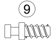
(x16) #A22910 connector bolt
