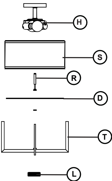
DRAWING 3- Shade installation
