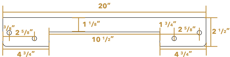
FRENCH MOUNTING BRACKET
