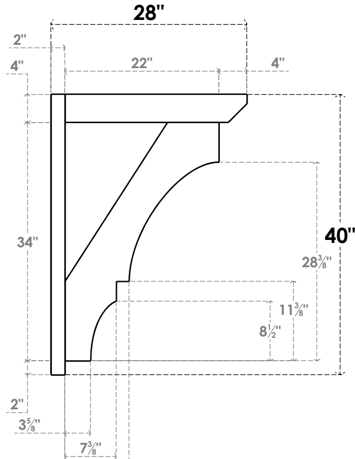
SIDE PROFILE
