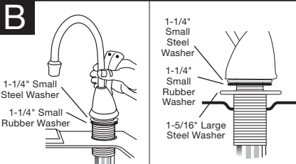
Standard 1-1/2" hole
