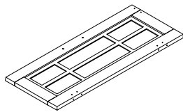
14 (614X252X15mm)X1
