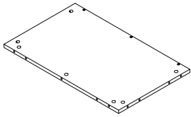
1 (620X385X15mm)X1
