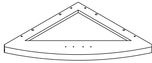
6 (440X440X30mm)X1
