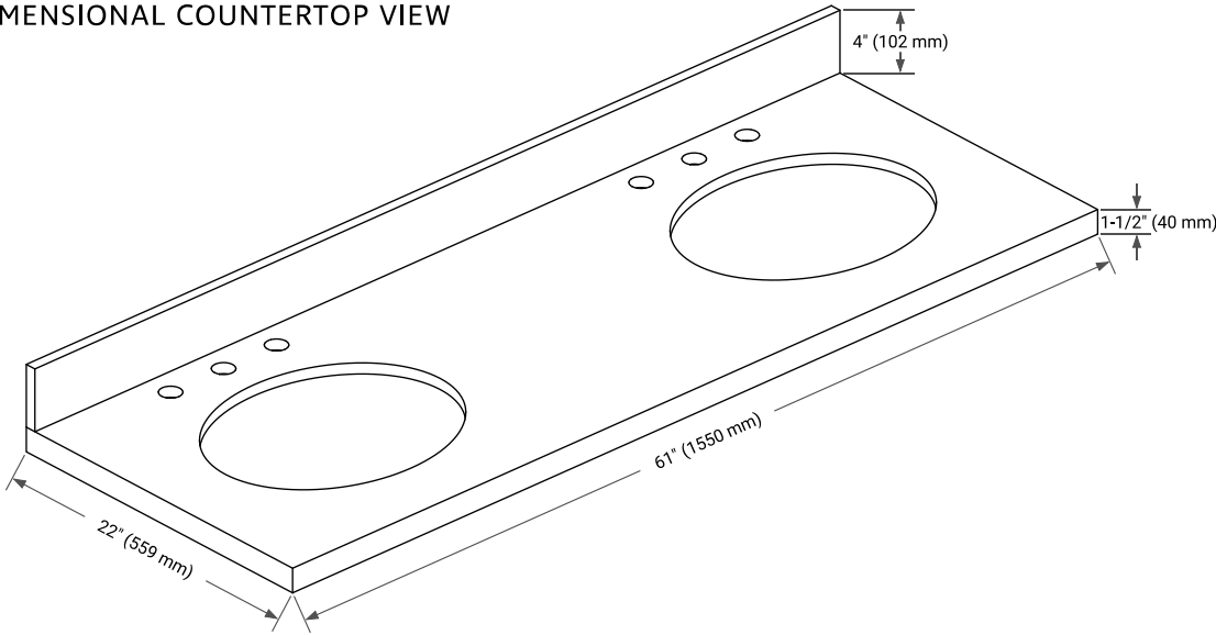
THREE DIMENSIONAL COUNTERTOP VIEW
