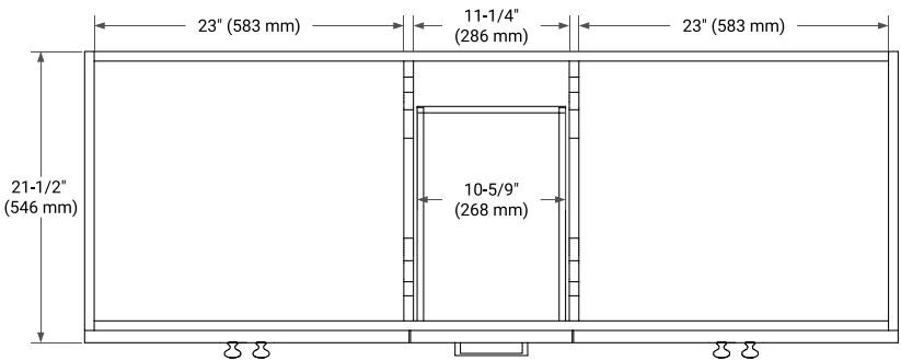
PLAN VIEW
