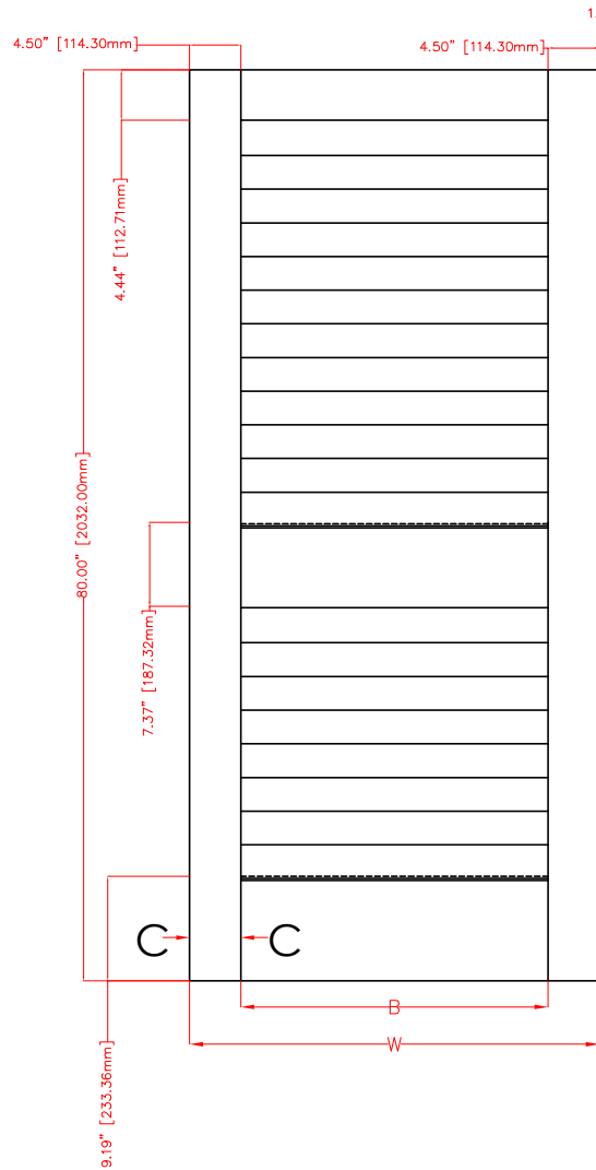
LVR SECTION Scale 6:1
