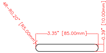
LVR SECTION Scale 6:1
