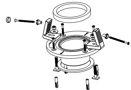
Flange, Sealing Wax Rings, Mounting Accessory Kit
