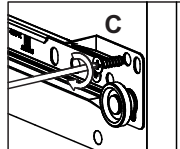
Drawer Lock
