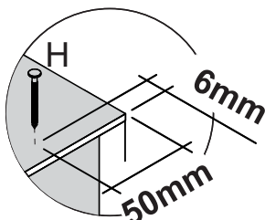
Detail 22
