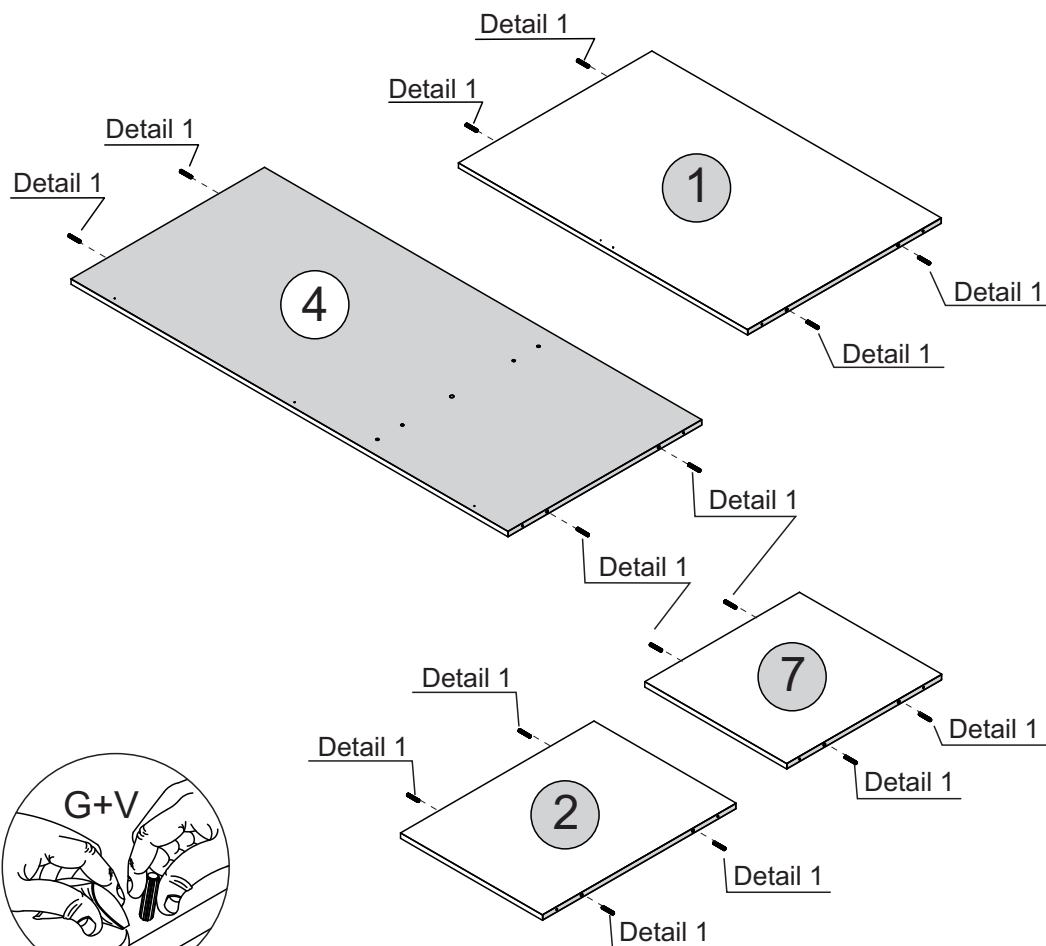
Detail 1
