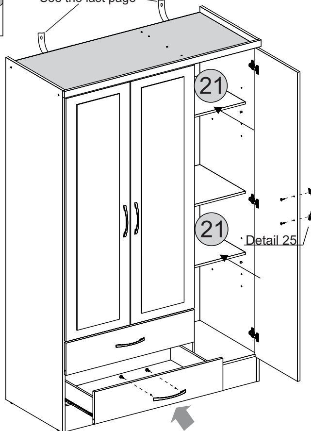
Height Adjustment
