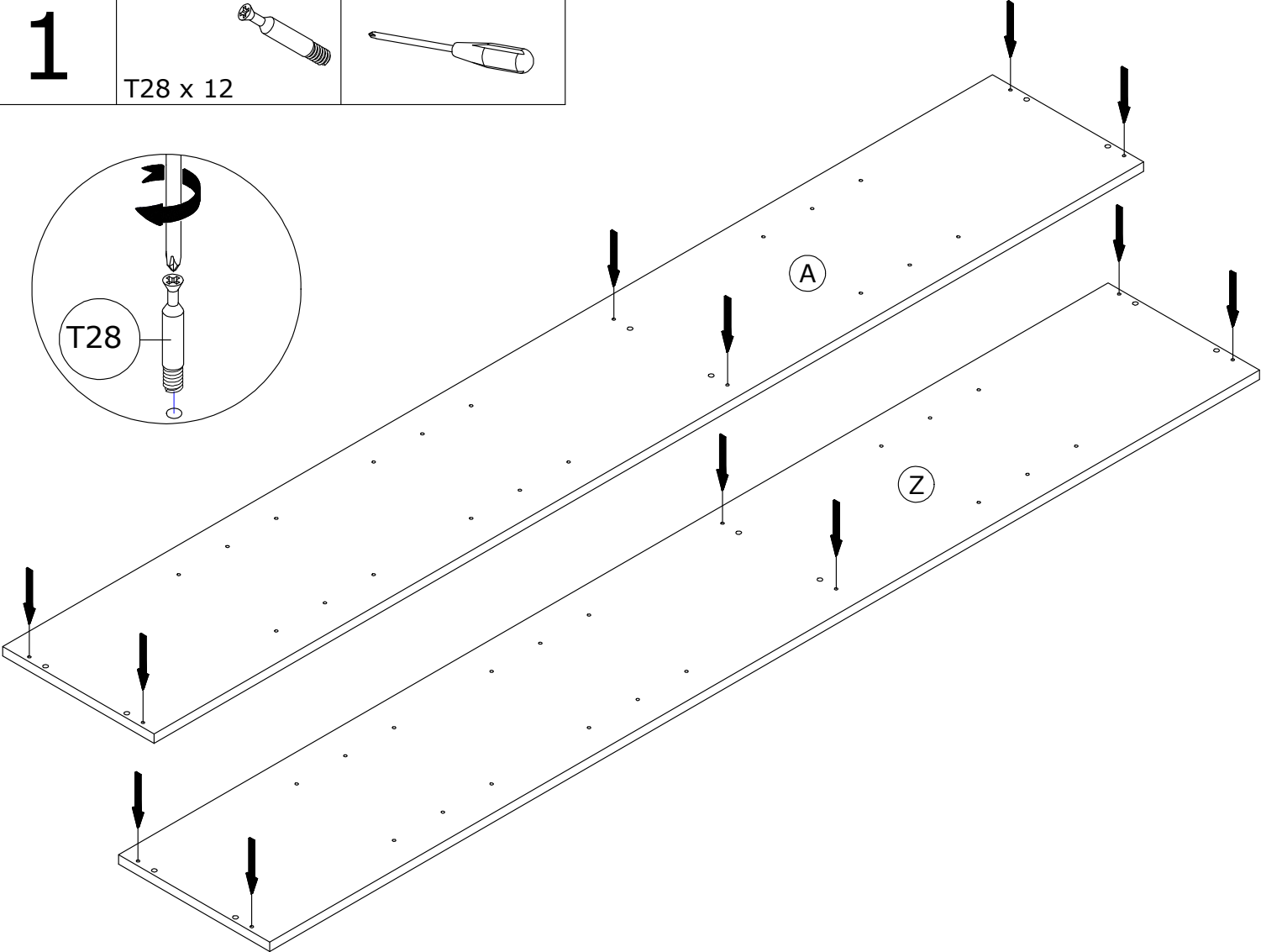
● FI6093 1950x298x16mm
