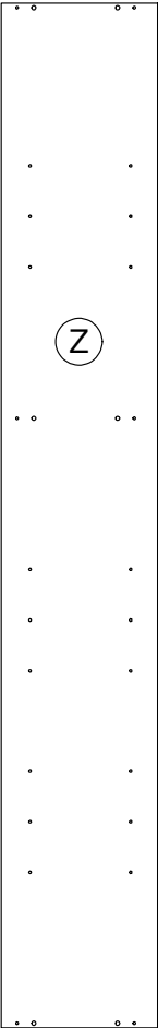
● FI6093 1950x298x16mm
