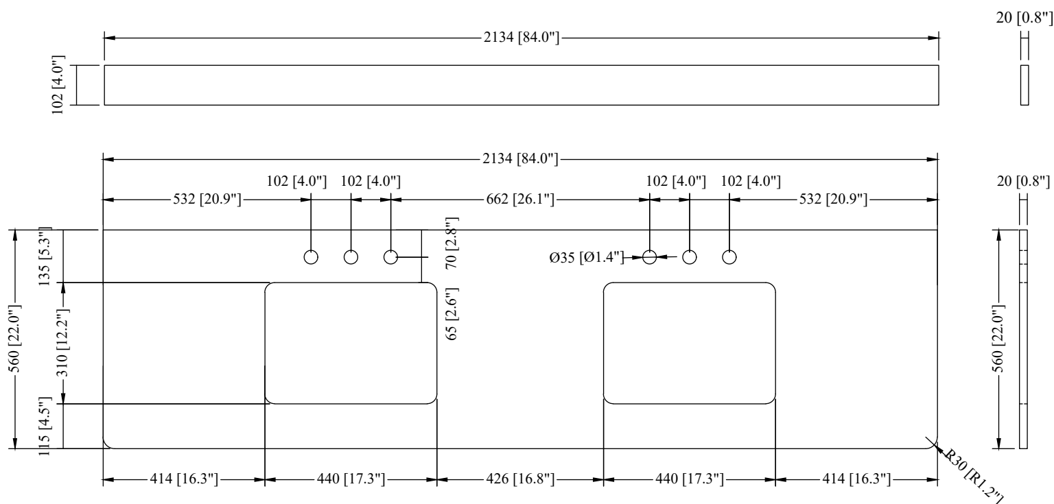
VanityTop
