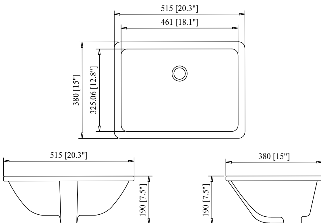
Undermount Sink
