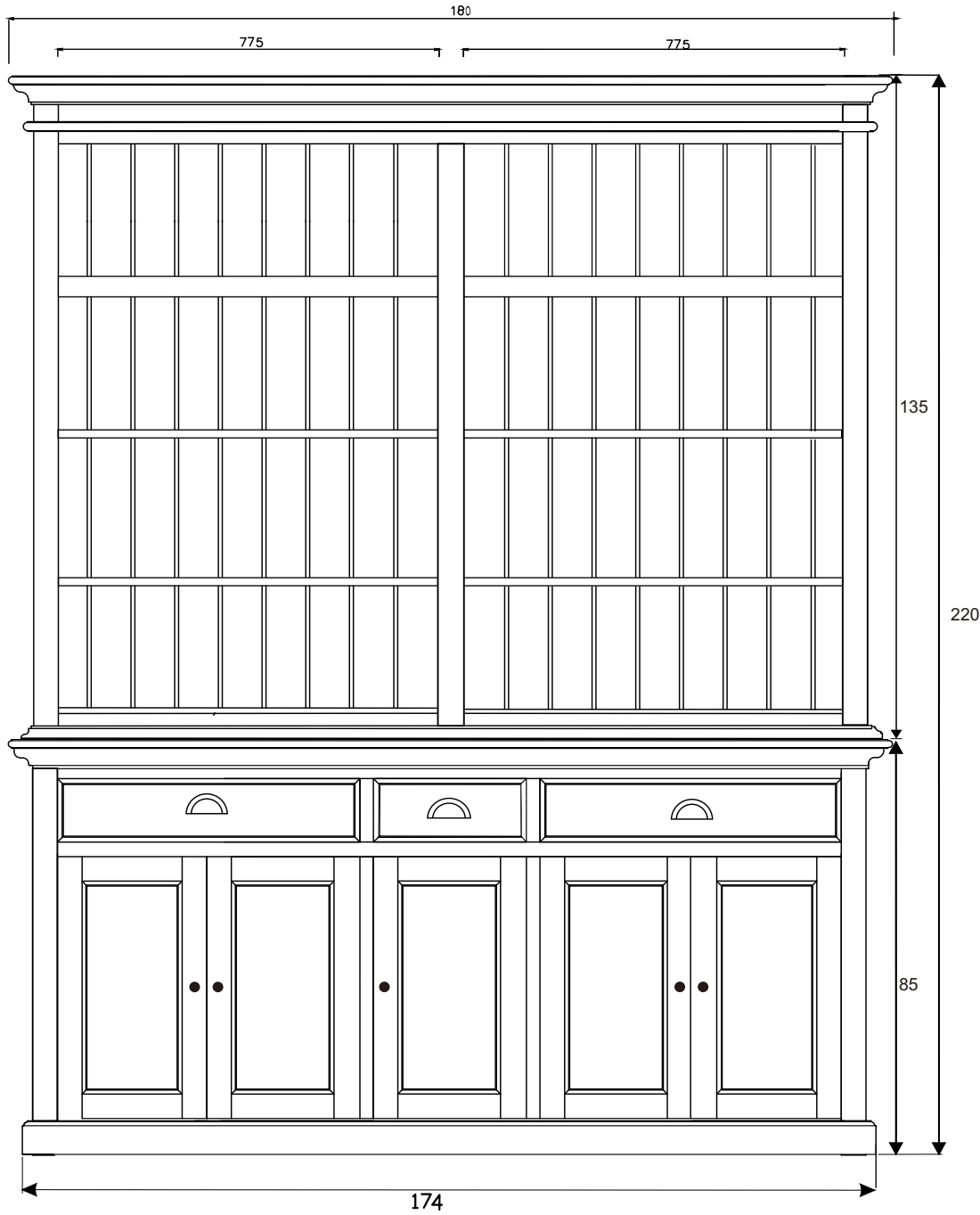
FRONT VIEW
