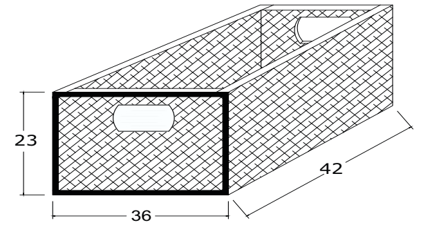
DETAIL BASKET
