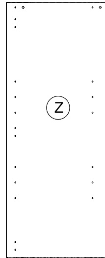
1050x423x22mm
