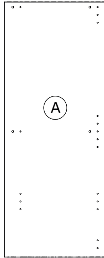
1050x423x22mm
