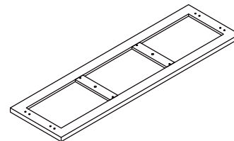
Ⓗ Top Panel X 1
