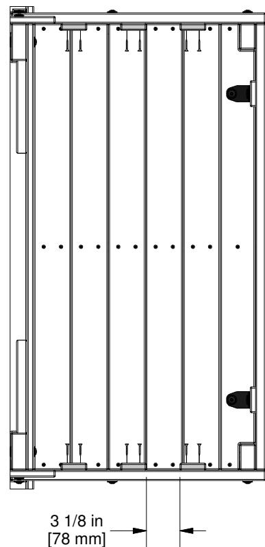
TOP VIEW
