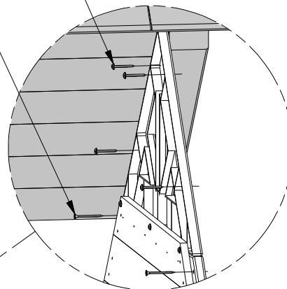
180 (x8) SCREW - 1-1/4
