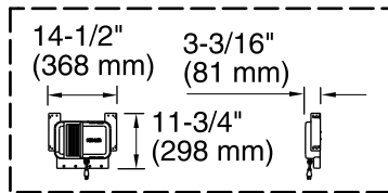
Control Amplifier
