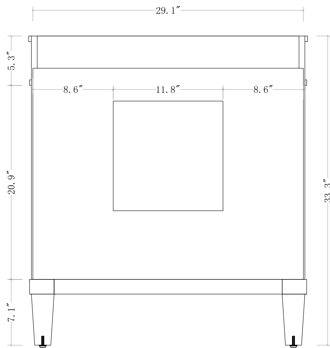
BACK VIEW
