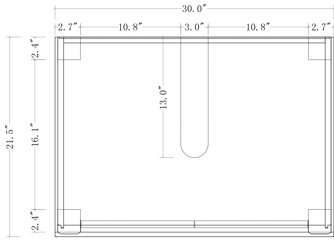
TOP VIEW
