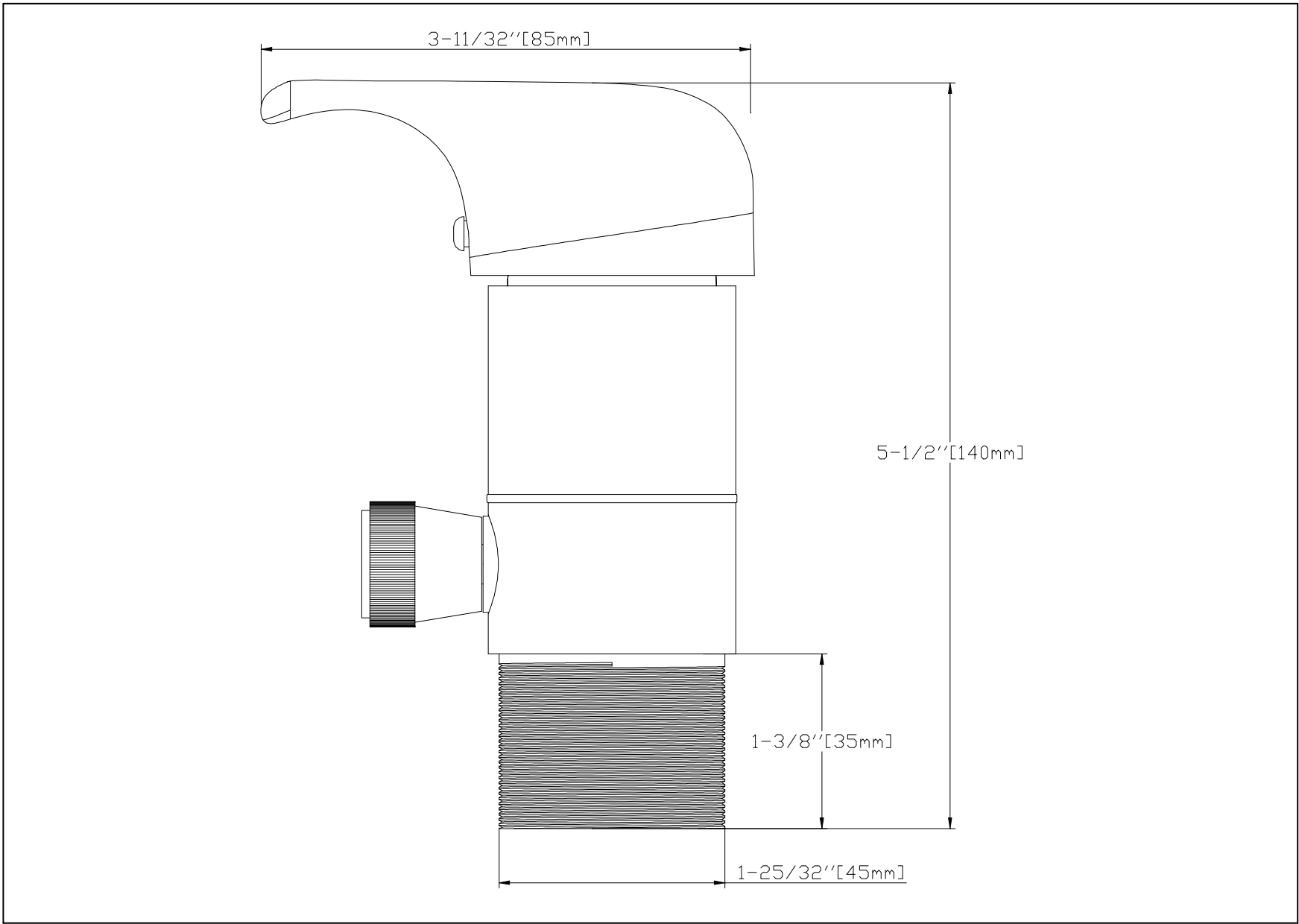
SIDE VIEW
