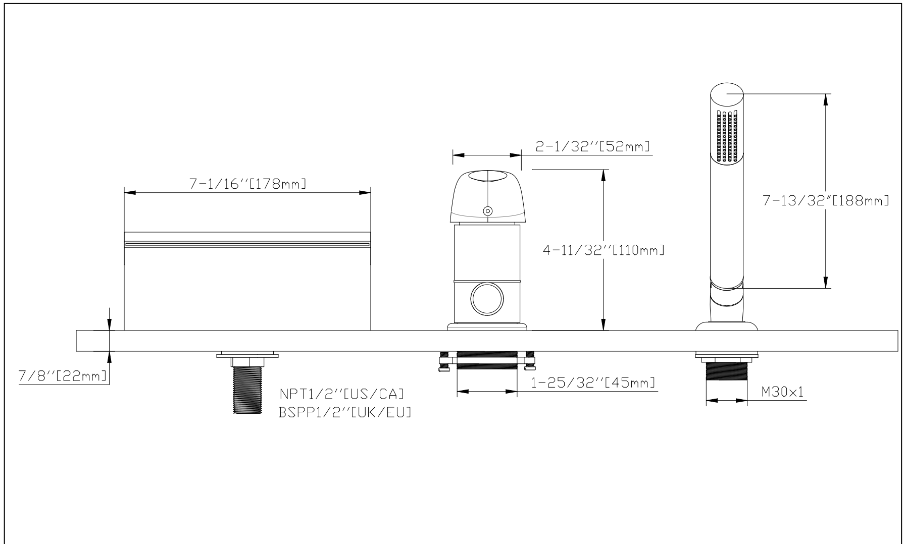
FRONT VIEW
