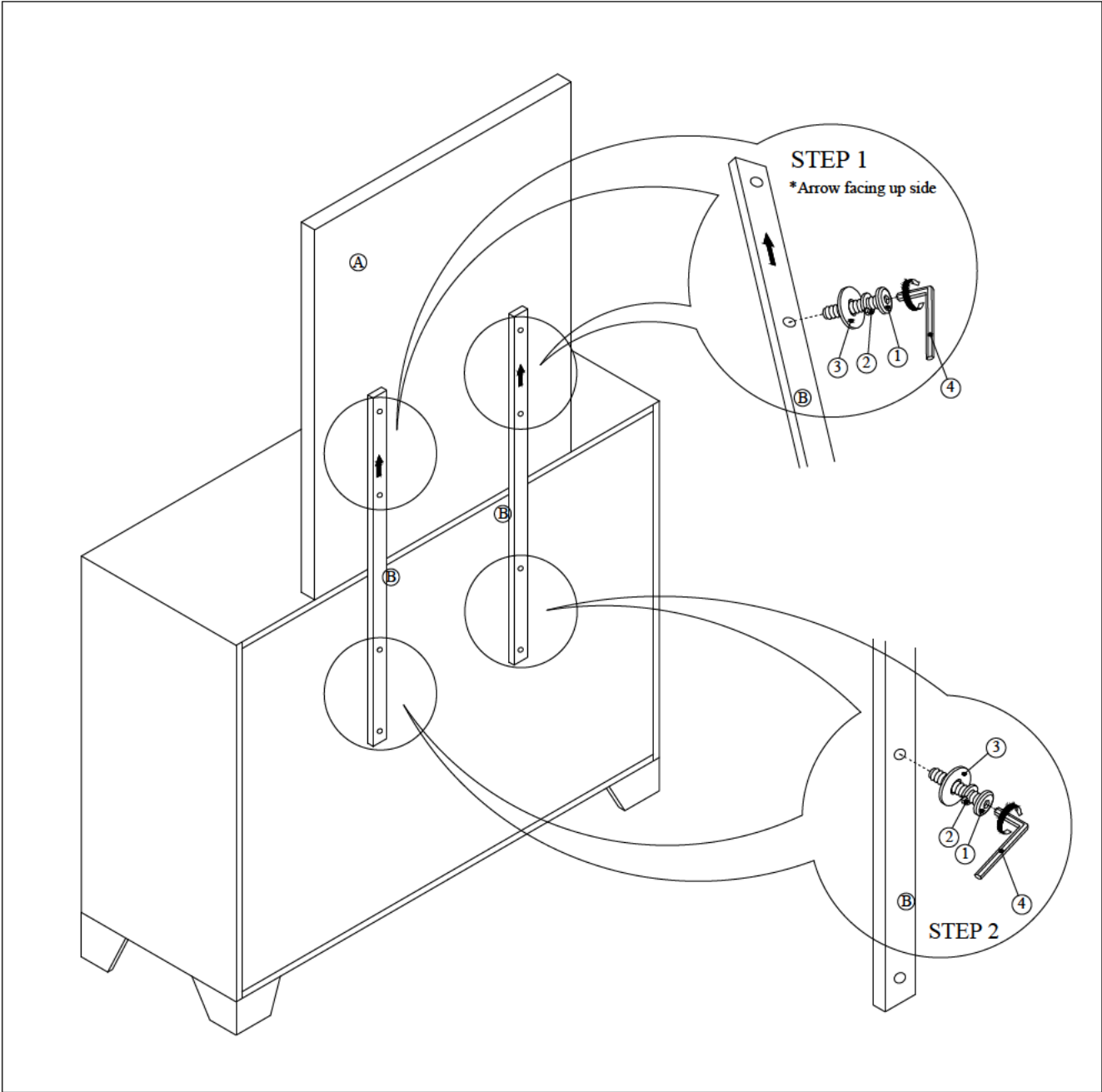
COMPLETED MIRROR ASSEMBLY
