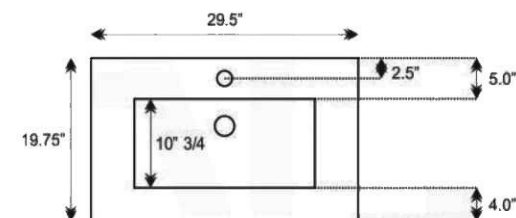
SINK CUT OUT OPENING 15.75"W x 10.75"D
