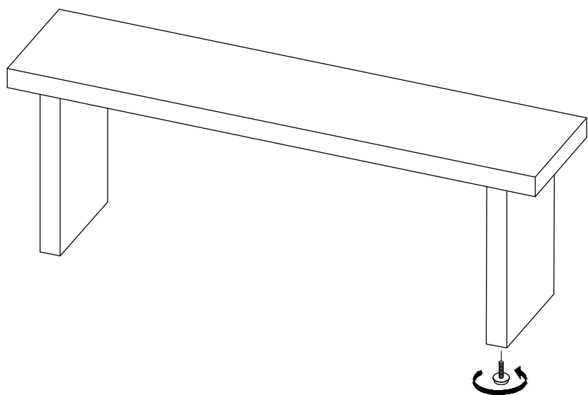
Adjustable Leveler
